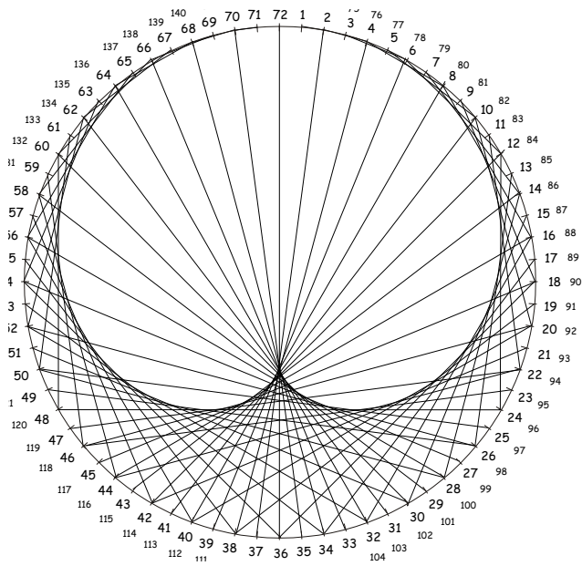
n → 2 n kardioda
